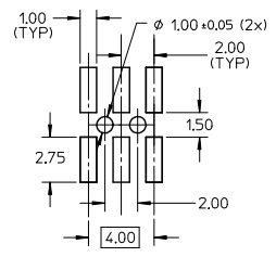
RECOMMENDED PCB PATTERN
