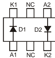
Internal Schematic
