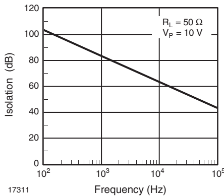
Fig. 12 - Output Isolation
