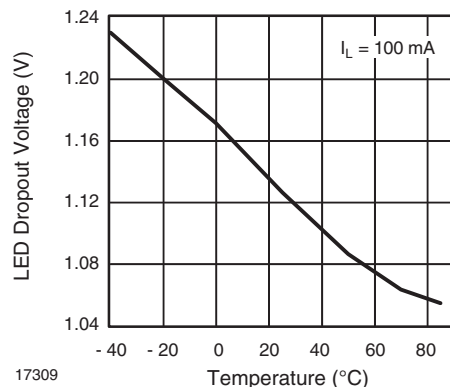
Fig. 10 - LED Dropout Voltage vs. Temperature
