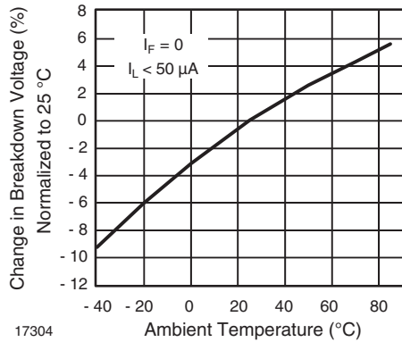
Fig. 5 - Switch Breakdown Voltage vs. Temperature
