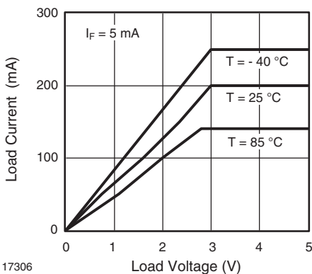
Fig. 7 - Load Current vs. Load Voltage
