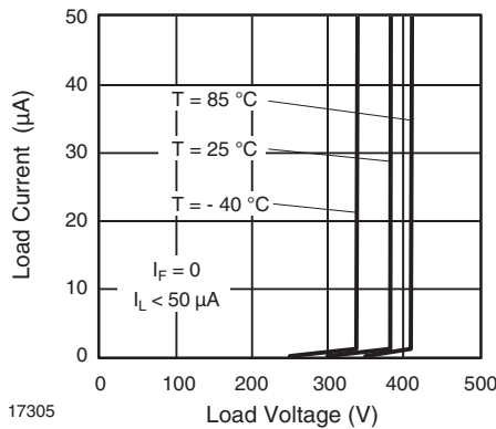
Fig. 6 - Switch Breakdown Voltage vs. Load Current
