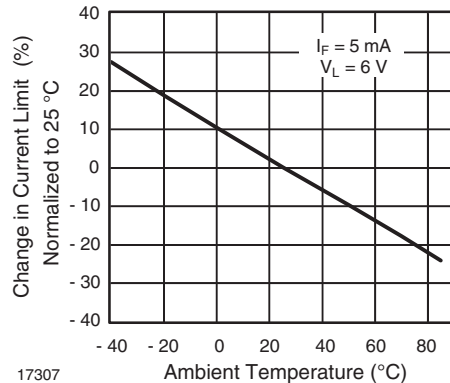
Fig. 8 - Current Limit vs. Temperature
