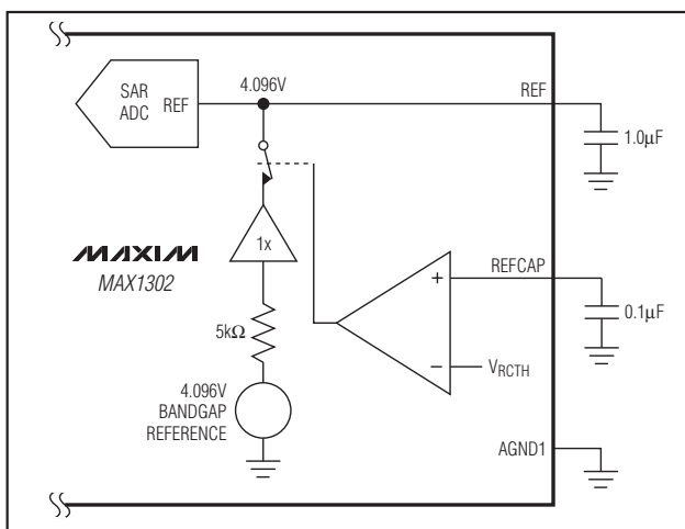
Figure 17. Internal Reference Operation
