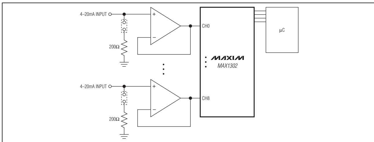
Figure 19. 4-20mA Application
