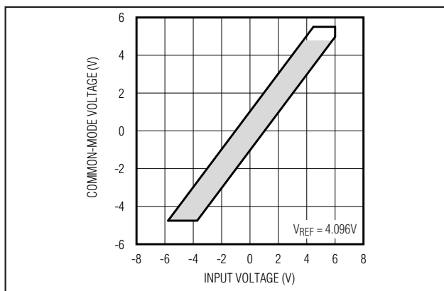
Figure 9. Common-Mode Voltage vs. Input Voltage (FSR = V_{REF} )
