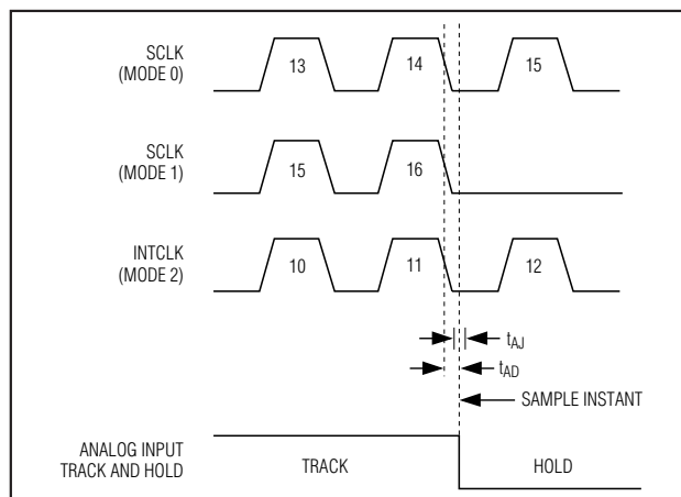
Figure 21. Aperture Diagram
