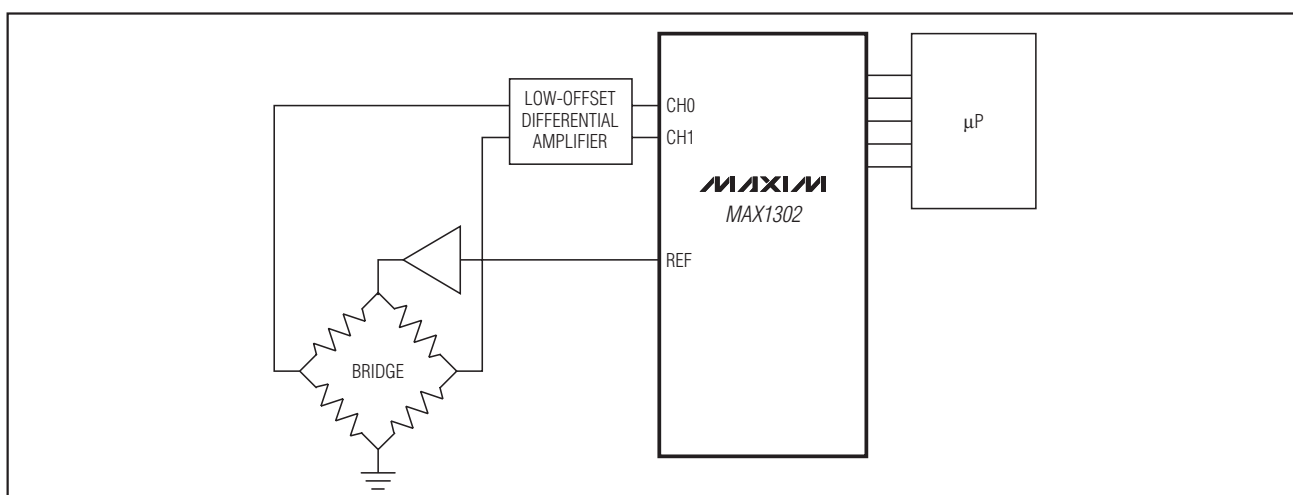
Figure 20. Bridge Application
