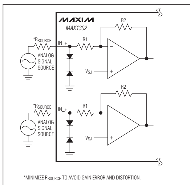
Figure 6. Simplified Analog Input Circuit
