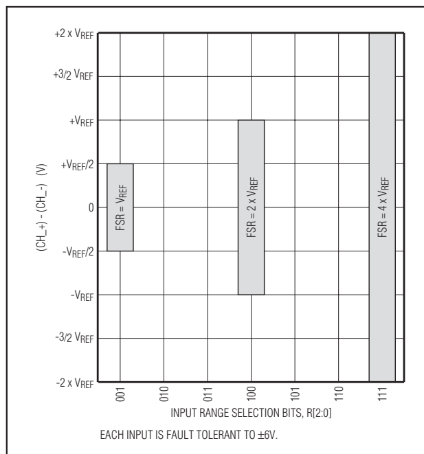
Figure 8. Differential Input Voltage Ranges
