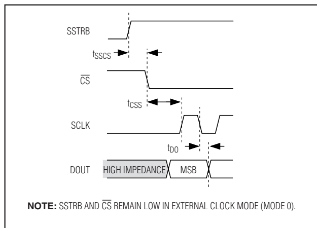
Figure 16. DOUT and SSTRB Timing
