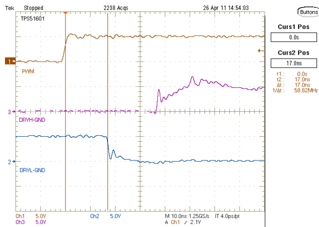
Figure 1. PWM Rising to DRVH Falling
