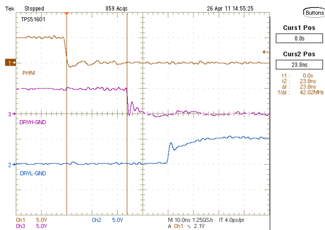
Figure 3. PWM Falling to DRVH Falling
