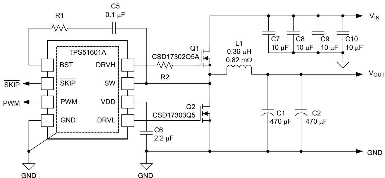
Figure 19. Typical Application
