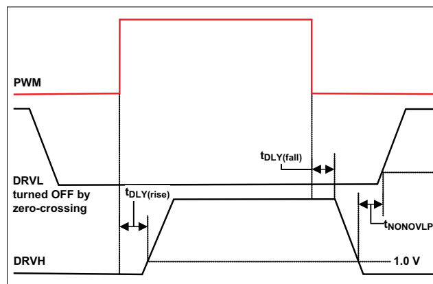
Figure 18. Discontinuous Conduction Mode Waveforms
