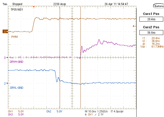
Figure 2. DRVH Falling to DRVH rising
