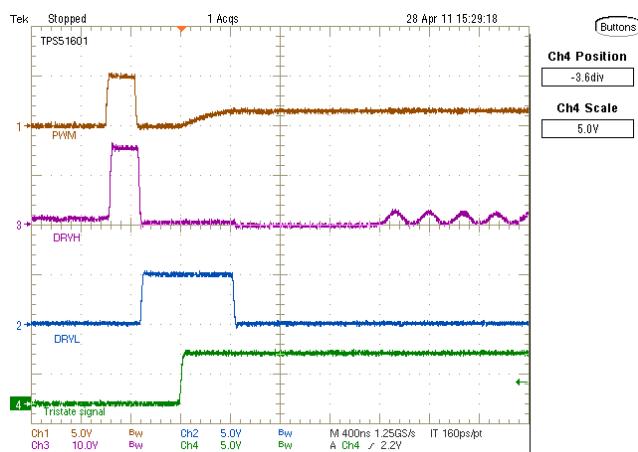
Figure 5. 3-State Entry on DRVH
