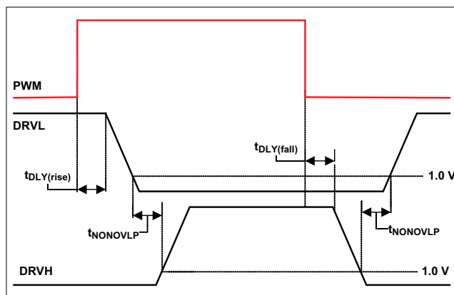
Figure 17. Continuous Conduction Mode Waveforms
