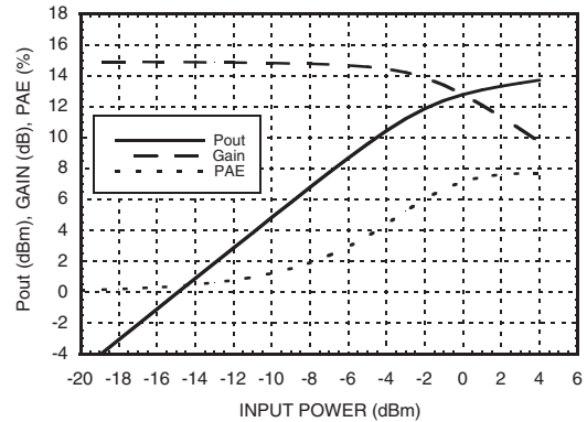
Power Compression @ 6 GHz
