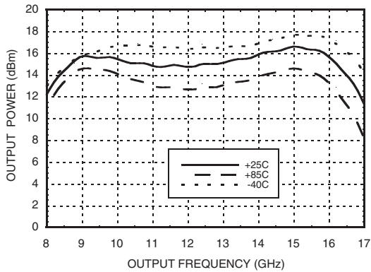
Output Power vs. Temperature @ +2 dBm Drive Level
