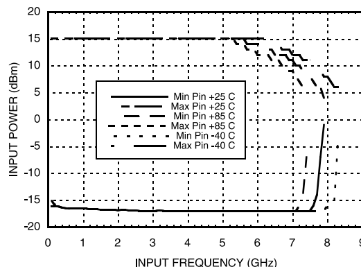
Input Sensitivity Window vs. Temperature
