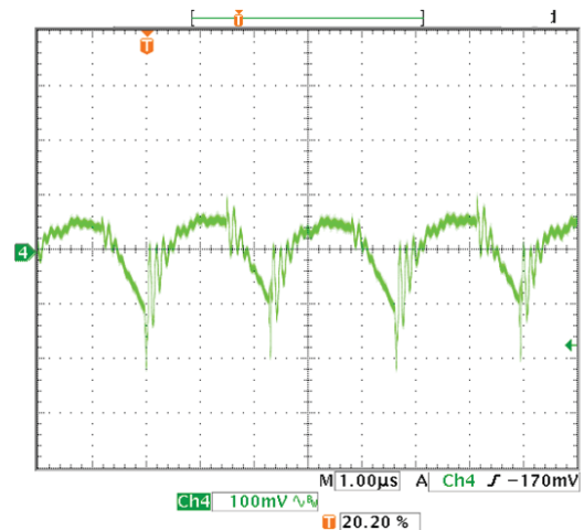
Output Ripple and Noise (Vin=48V, Vout=nom, Iout=3A, Cload=1uF, Ta=+25°C)
