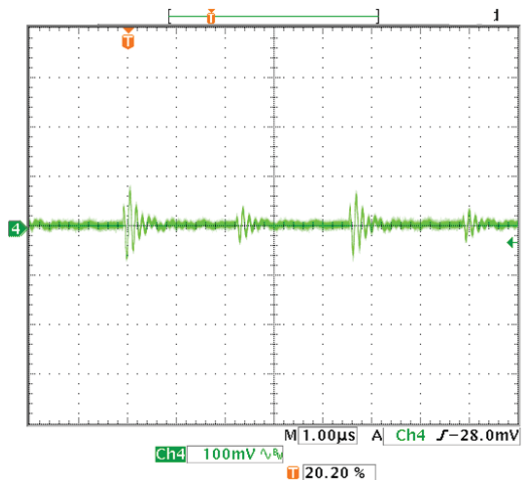
Output Ripple and Noise (Vin=48V, Vout=nom, Iout=0A, Cload=1uF, Ta=+25°C)
