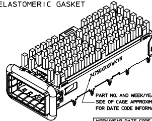
QSFP CAGE W/ ELASTOMERIC GASKET
