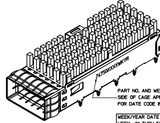
QSFP CAGE W/ EMI SPRING FINGERS
