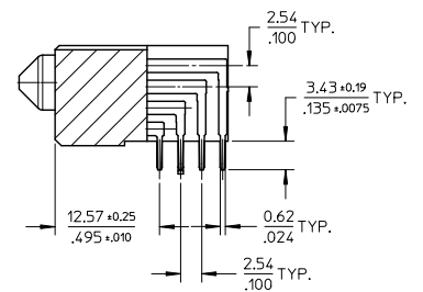
SECTION Y-Y
