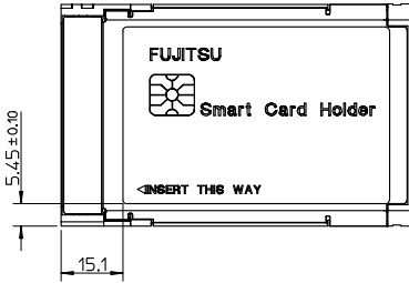
METAL COVER SIDE LABEL PART NUMBER 90848-0460 OR 90848-0462
