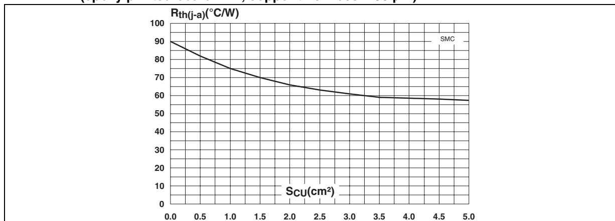
Figure 11. Thermal resistance junction to ambient versus copper surface under each lead (epoxy printed board FR4, copper thickness = 35 \mu\text{m} )
