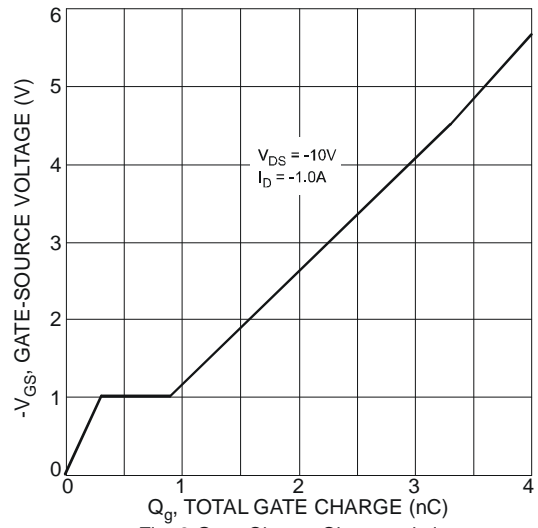
Fig. 8 Gate-Charge Characteristics
