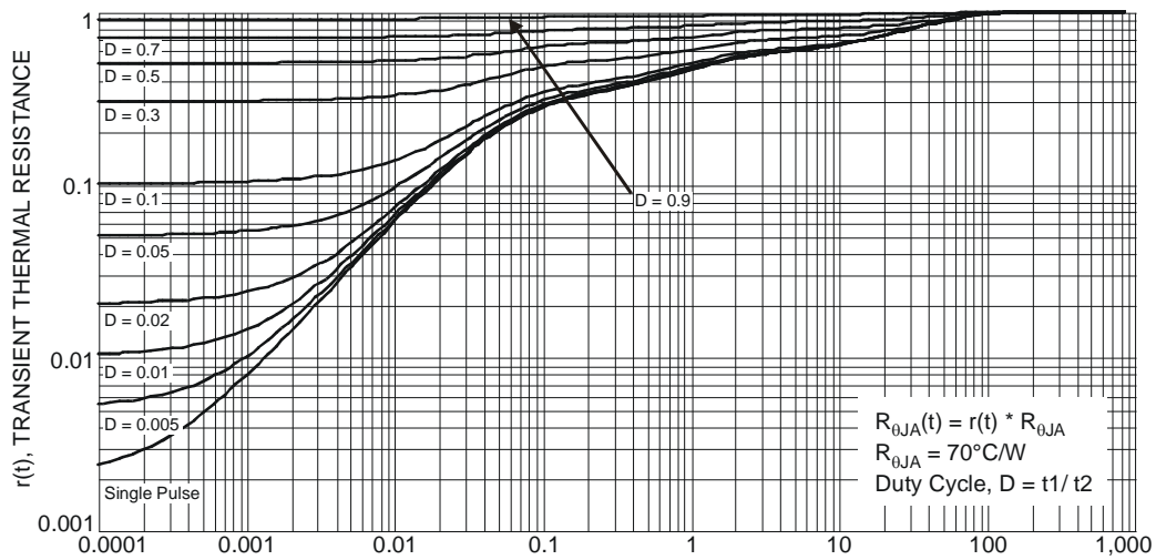
Fig. 10 Transient Thermal Resistance
