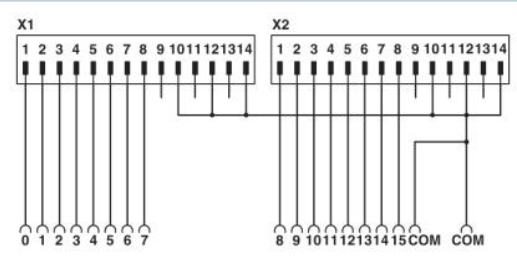
Connection scheme FLKM 14-PA-SLC500/IN
