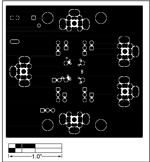
Figure 4. MAX3558 EV Kit PC Board Layout—Ground Plane 1
