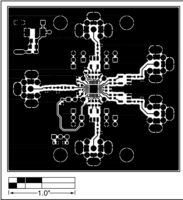
Figure 3. MAX3558 EV Kit PC Board Layout—Component Side
