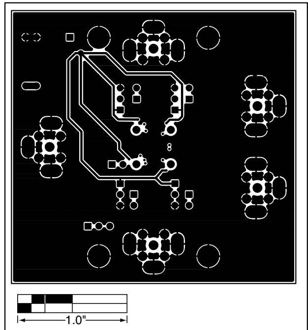
Figure 6. MAX3558 EV Kit PC Board Layout—Solder Side
