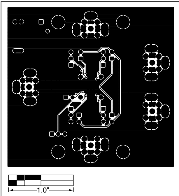
Figure 5. MAX3558 EV Kit PC Board Layout—Ground Plane 2
