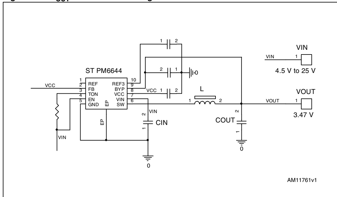
Figure 1. V_{OUT} = 3.47\text{ V} fixed configuration
