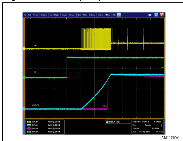
Figure 10. Power-up sequence, no load
