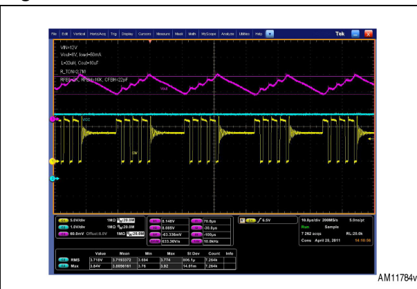
Figure 25. Load = 50 mA
