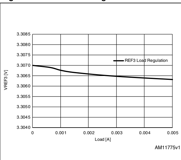
Figure 15. VREF3 load regulation
