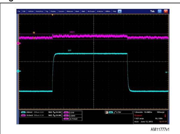
Figure 17. VREF3 line transient
