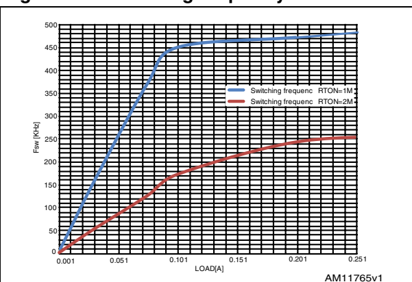
Figure 5. Switching frequency vs. load
