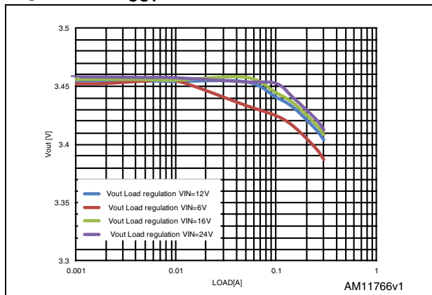
Figure 6. V_{OUT} vs. load
