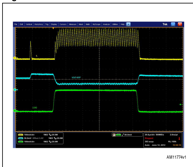
Figure 14. Load transient 0-200 mA
