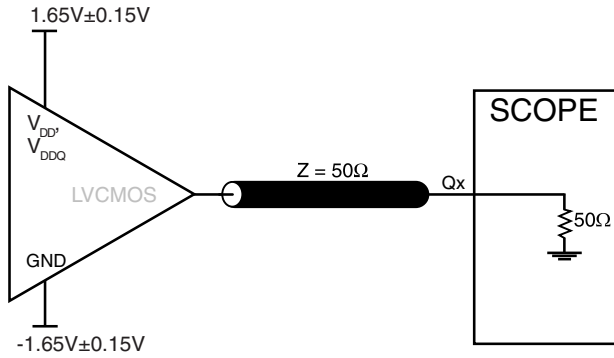
3.3V CORE/3.3V OUTPUT LOAD ACT TEST CIRCUIT
