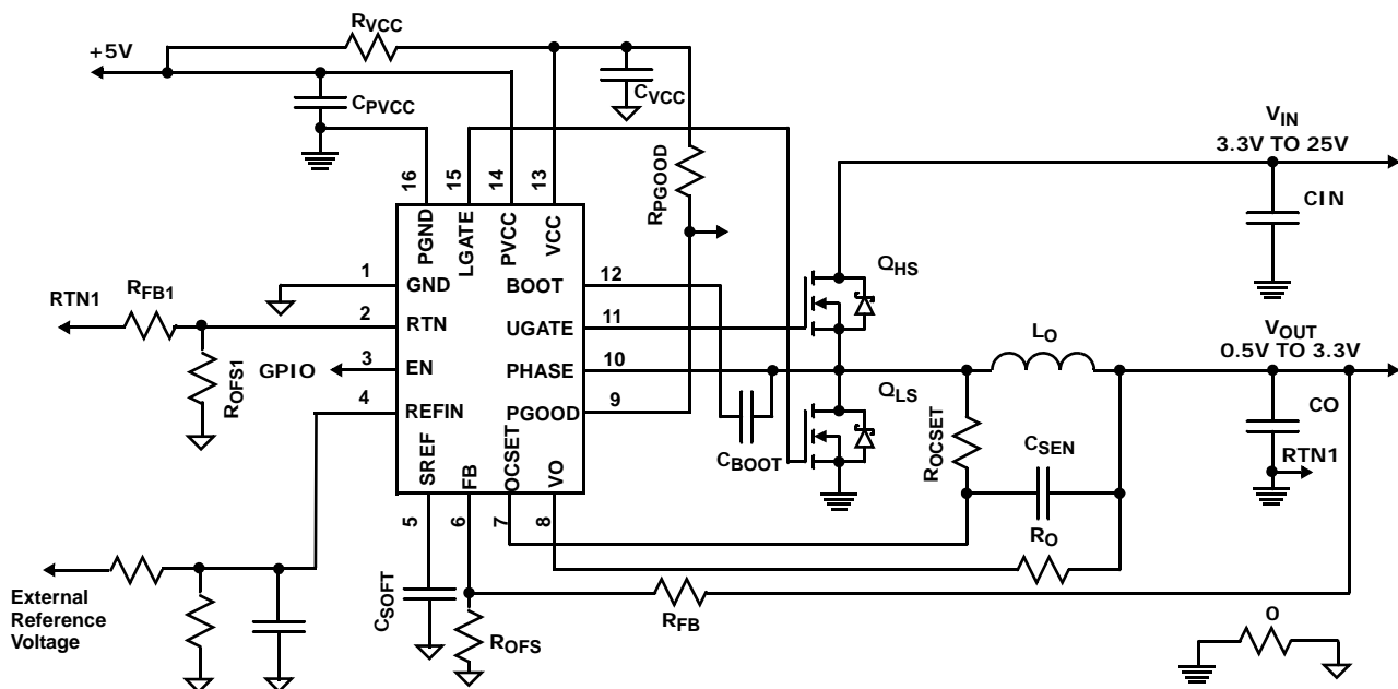
FIGURE 1. ISL95872 APPLICATION SCHEMATIC WITH DCR CURRENT SENSE
