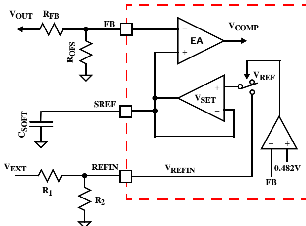
FIGURE 5. REFIN CONNECTION TO SYSTEM RAIL
