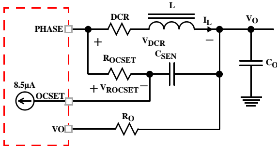
FIGURE 13. OVERCURRENT PROGRAMMING CIRCUIT
