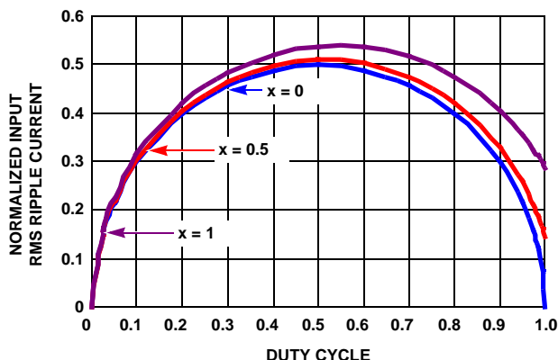
FIGURE 15. NORMALIZED INPUT RMS CURRENT FOR EFF = 1
