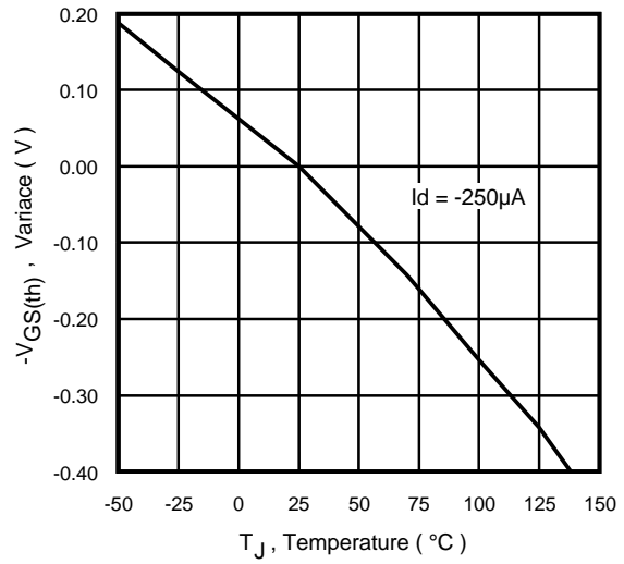
Fig 10. Typical V_{GS(th)} Variance Vs. Junction Temperature
