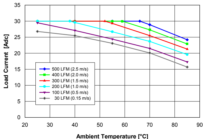
Fig. 10: Available load current vs. ambient air temperature and airflow rates for converter mounted vertically with V_{in} = 27 V, air flowing from pin 3 to pin 1 and maximum FET temperature \leq 120^{\circ}\text{C} .
