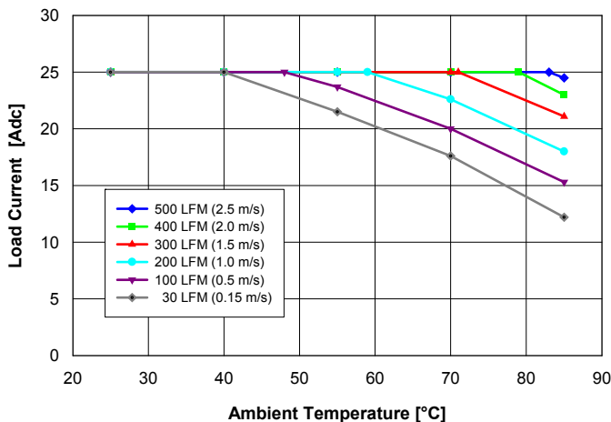
Fig. 1: Available load current vs. ambient air temperature and air-flow rates for Q48T25033 converter mounted vertically with air flowing from pin 3 to pin 1, MOSFET temperature \leq 120^{\circ}\text{C} , V_{in} = 54\text{ V} .
