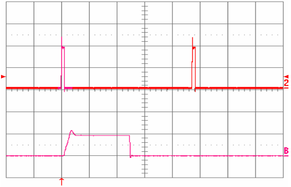
Fig. 26: Load current (top trace, 20 A/div, 20 ms/div) into a 10 mΩ short circuit during restart, at Vin = 48 V. Bottom trace (40 A/div, 1 ms/div) is an expansion of the on-time portion of the top trace.
