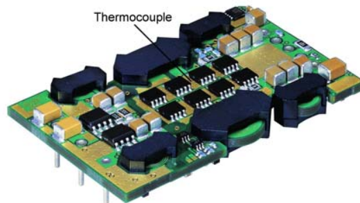
Fig. 27: Location of the thermocouple for thermal testing.
