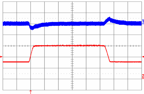
Fig. 19: Output voltage response to load current step-change (7.5 A – 15 A – 7.5 A) at V_{in} = 48\text{ V} . Top trace: output voltage (100 mV/div). Bottom trace: load current (5 A/div.). Current slew rate: 0.1 A/ \mu\text{s} . C_o = 1\ \mu\text{F} ceramic. Time scale: 0.2 ms/div.
