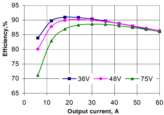
Figure 3. HHS60ZB (1.8V) Efficiency Curves
