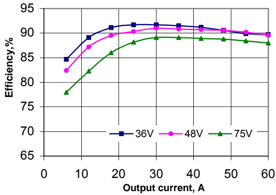
Figure 1. HHS60ZE, (3.3V) Efficiency Curves
