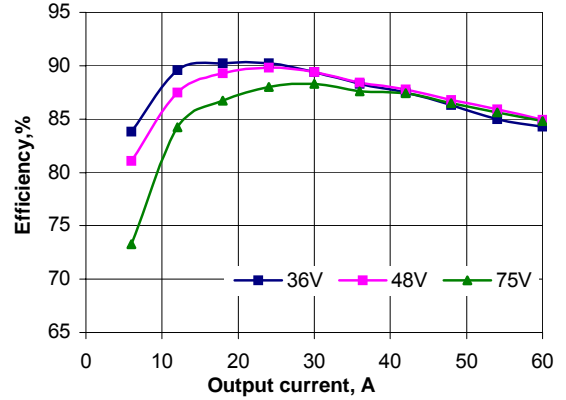
Figure 4. HHS60ZA (1.5V) Efficiency Curves
