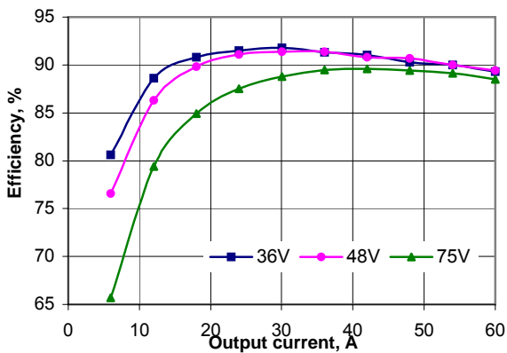
Figure 2. HHS60ZD (2.5V) Efficiency Curves
