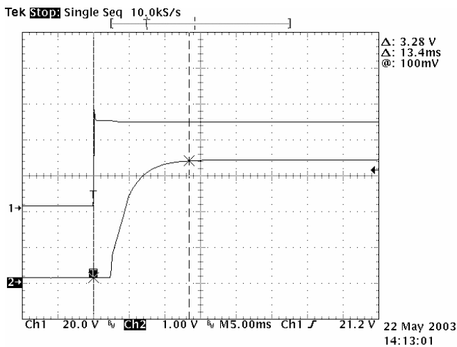
Figure 10. Output Voltage turn-on HHS60ZE Conditions: Vin=48V, Load: full, Co=none
