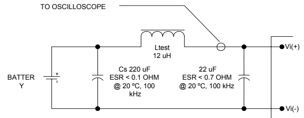
Figure 18. Input Reflected Ripple Current Test Setup
