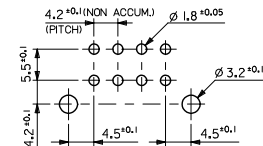
RECOMMENDED PCB HOLE LAYOUT VIEWED FROM COMPONENT SIDE 1.78 MAX. THICK P.C. BOARD
