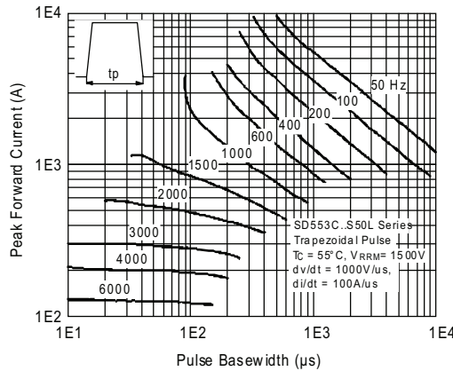
Fig. 20 - Frequency Characteristics
