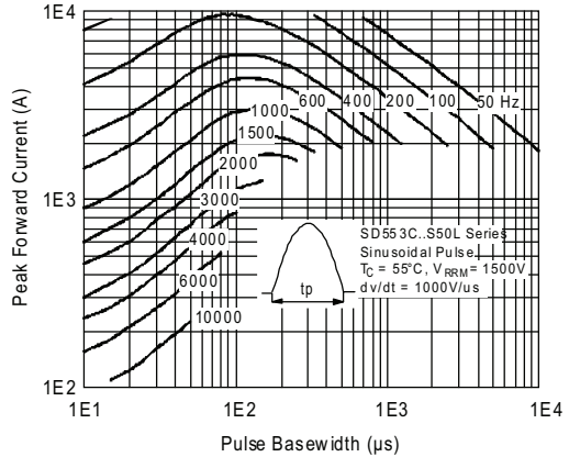
Fig. 16 - Frequency Characteristics
