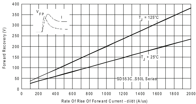
Fig. 11 - Typical Forward Recovery Characteristics
