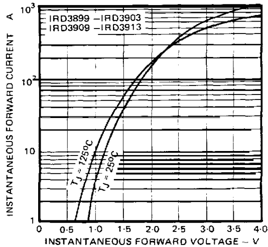
Fig. 4 - Maximum Forward Voltage Vs. Forward Current, Both Series
