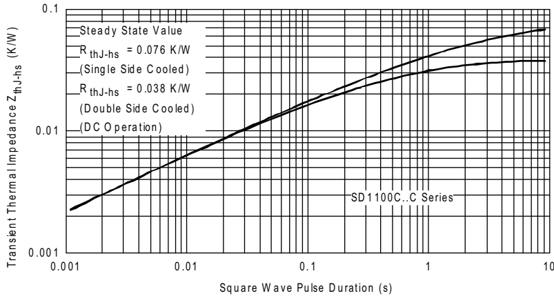
Fig. 19 - Thermal Impedance Z_{thJ-hs} Characteristics
