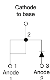
TO-247AC modified
