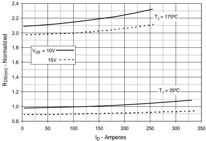
Fig. 5. R_{DS(on)} Normalized to I_D = 125\text{A} Value vs. Drain Current
