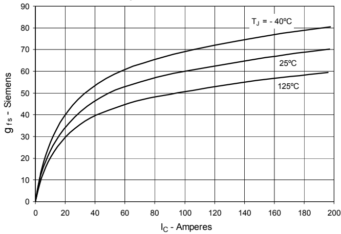
Fig. 7. Transconductance
