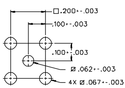
MOUNTING HOLE LAYOUT
