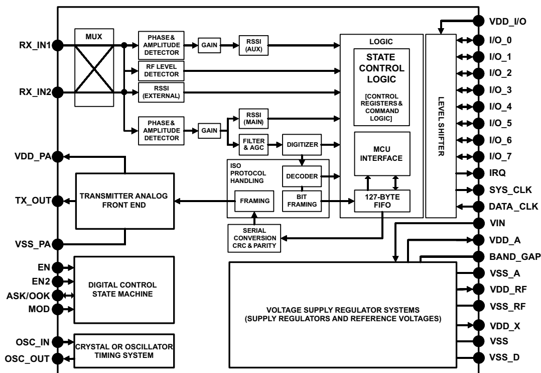
Figure 6-2. System Block Diagram
