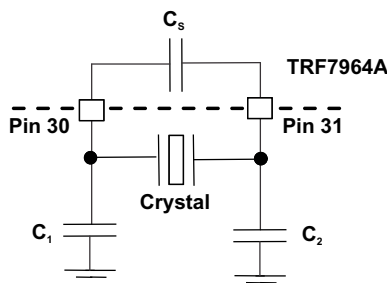
Figure 6-7. Crystal Block Diagram
