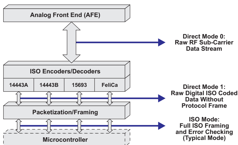
Figure 6-27. User-Configurable Modes
