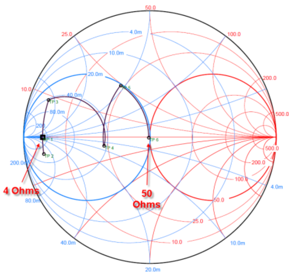
Figure 7-4. Smith Chart Simulation
