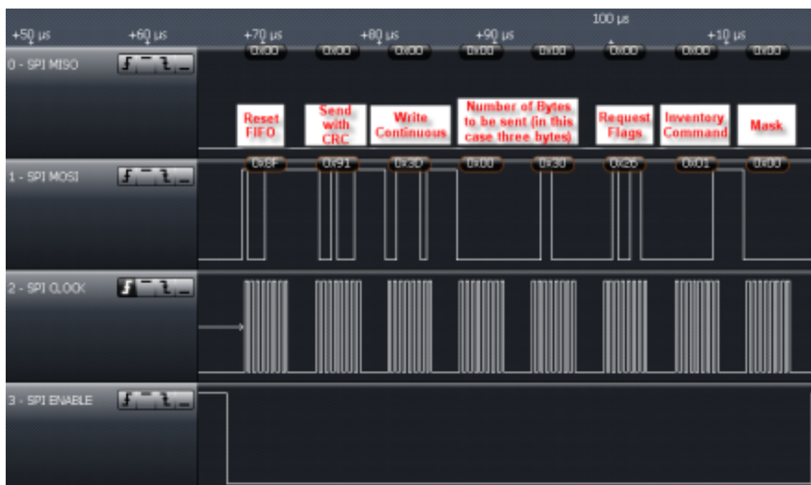
Figure 6-22. Inventory Command Sent From MCU to TRF7964A
