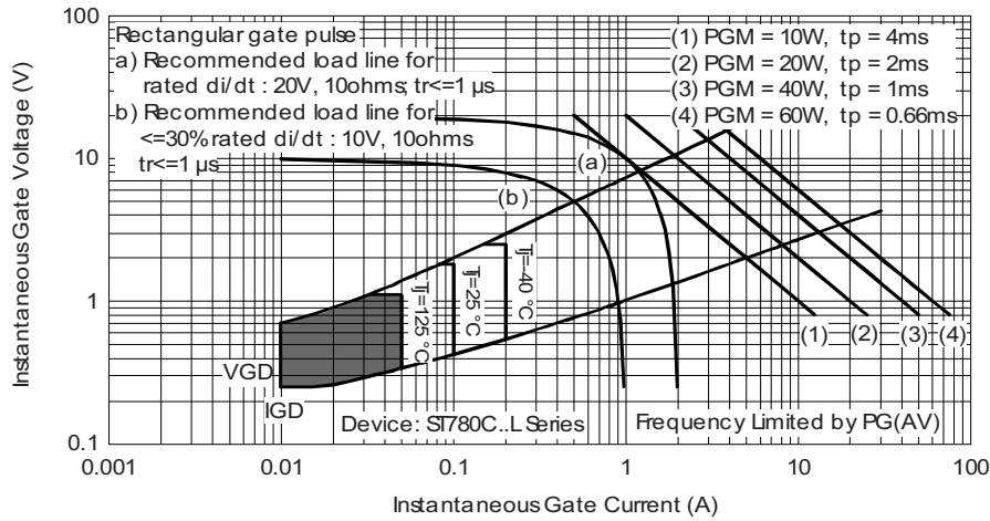
Fig. 11 - Gate Characteristics
