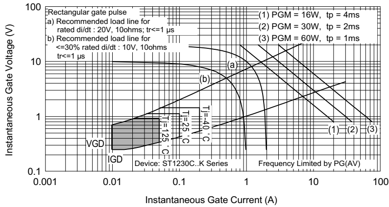
Fig. 11 - Gate Characteristics
