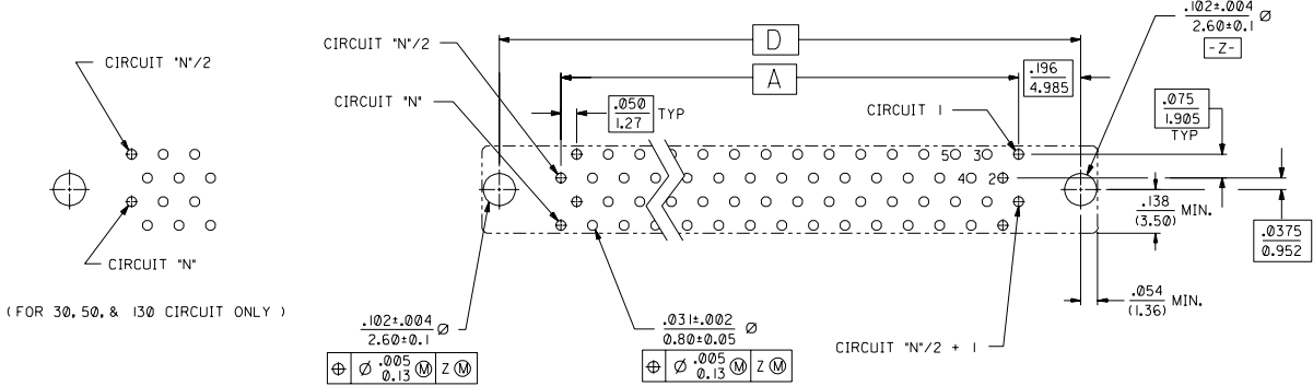
RECOMMENDED PC BOARD LAYOUT A COMPONENT SIDE (FOR 40, 60, 68, 80, 100, & 120 ONLY)
