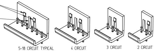
AUXILIARY VIEWS SCALE 1:1
