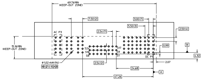
RECOMMENDED PC BOARD LAYOUT & KEEP-OUT ZONE
