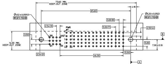
RECOMMENDED PCB LAY-OUT AND KEEP-OUT ZONE
