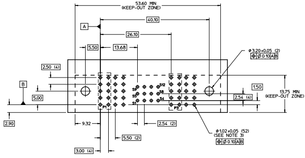
RECOMMENDED PCB LAYOUT AND KEEP-OUT ZONE
