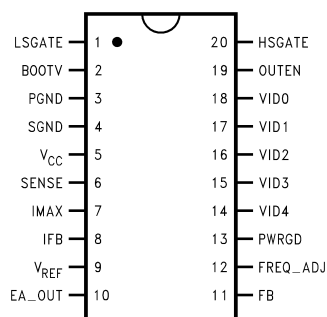
Figure 2. Plastic TSSOP-20 (Top View) See Package Number PW
