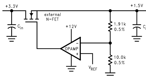
Figure 11. V_{REF} Used in an N-FET LDO Supply
