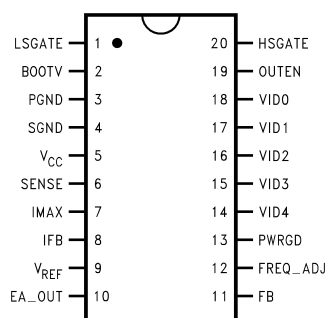
Figure 1. Plastic SOIC-20 (Top View) See Package Number DW
