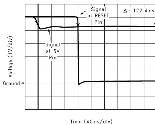
Figure 19. 5V Under-Voltage Waveforms
