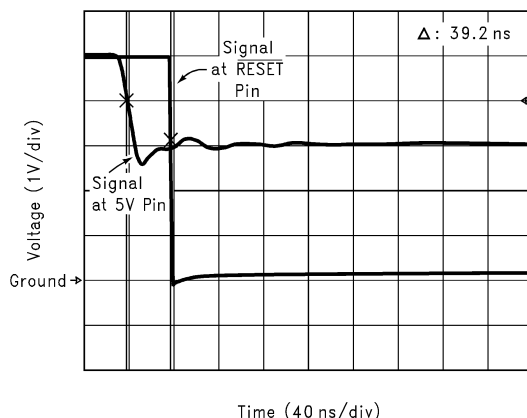
Figure 20. Power Failure Waveforms
