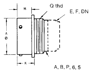
Crimp KPSE00/MS3120
