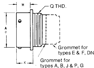
Crimp KPSE01/MS3121
