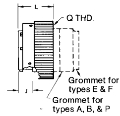
Crimp KPSE08
