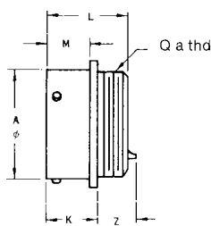
Solder KPT00/MS3110
