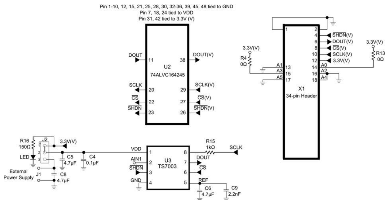
Figure 5. TS7003 Evaluation Board Circuit
