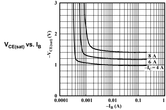
STD01P Performance Characteristics at T_A = 25^\circ\text{C}
