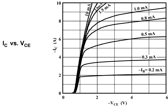
STD01P Performance Characteristics at T_A = 25^\circ\text{C}
