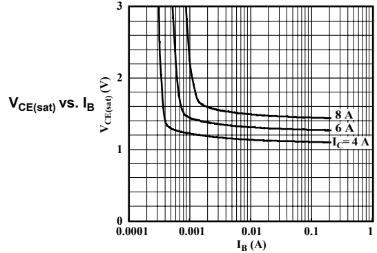
STD01N Performance Characteristics at T_A = 25^\circ\text{C}
