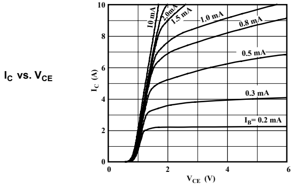
STD01N Performance Characteristics at T_A = 25^\circ\text{C}
