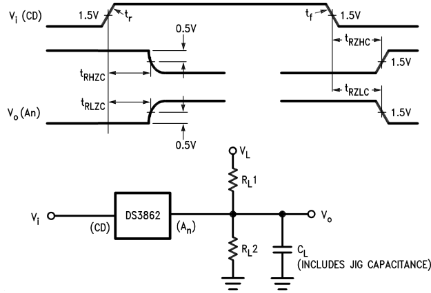
FIGURE 4. Propagation Delay From CD Pin to An
