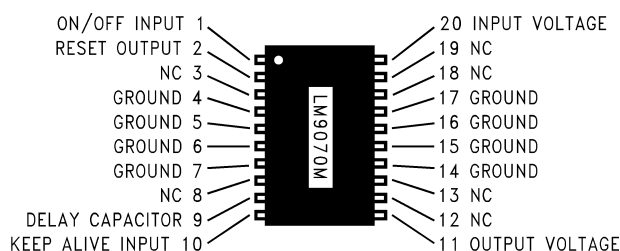
Figure 2. 20-Pin SOIC Package
