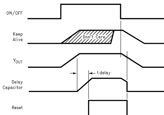
Figure 17. Simple ON/OFF control
