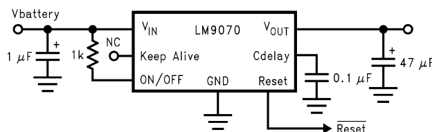
Figure 22. Control Logic Not Used
