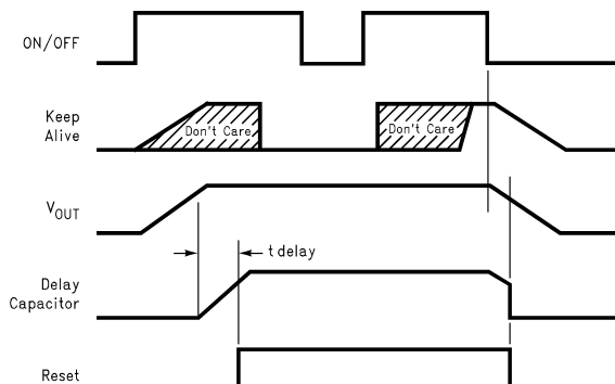
Figure 17. Simple ON/OFF control
