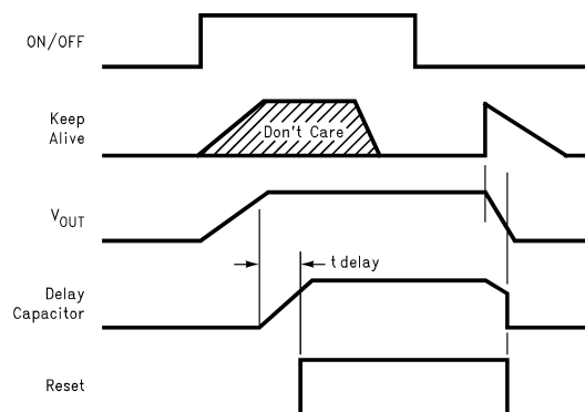
Figure 18. Keep-Alive Mode
