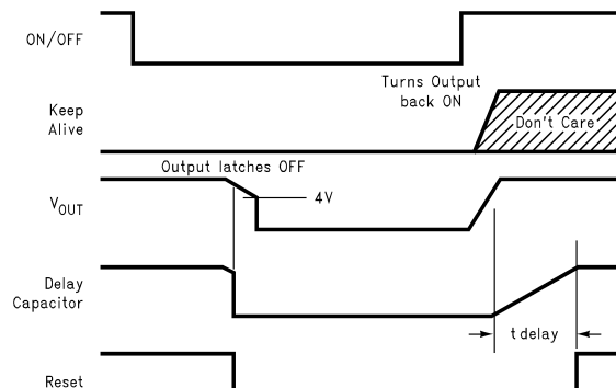
Figure 18. Keep-Alive Mode
