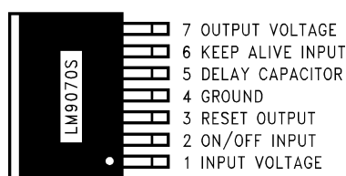
Figure 1. 7 Lead TO-263 (Top View) Package Number KTW0007B
