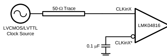
Figure 27. DC-Coupled LVCMOS and LVTTTL Reference Clock
