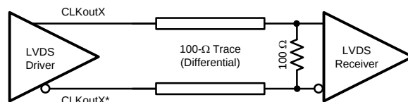
Figure 28. Differential LVDS Operation, DC Coupling, No Biasing of the Receiver
