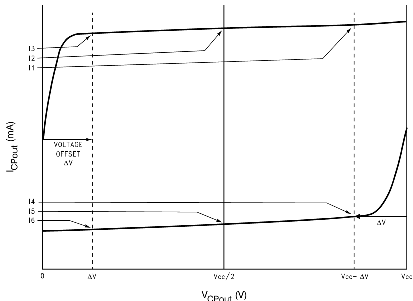
Figure 4. Charge-Pump Current
