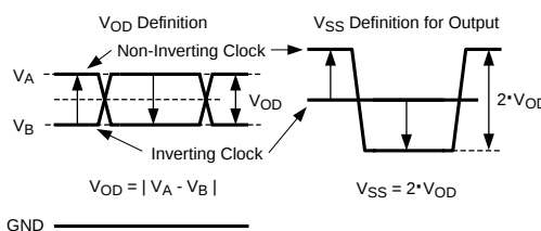
Figure 6. Two Different Definitions for Differential Output Signals
