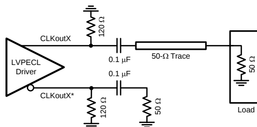
Figure 36. Single-Ended LVPECL Operation, AC Coupling
