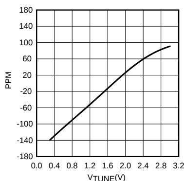
Figure 38. Example Tuning Curve, 20.48-MHz Crystal
