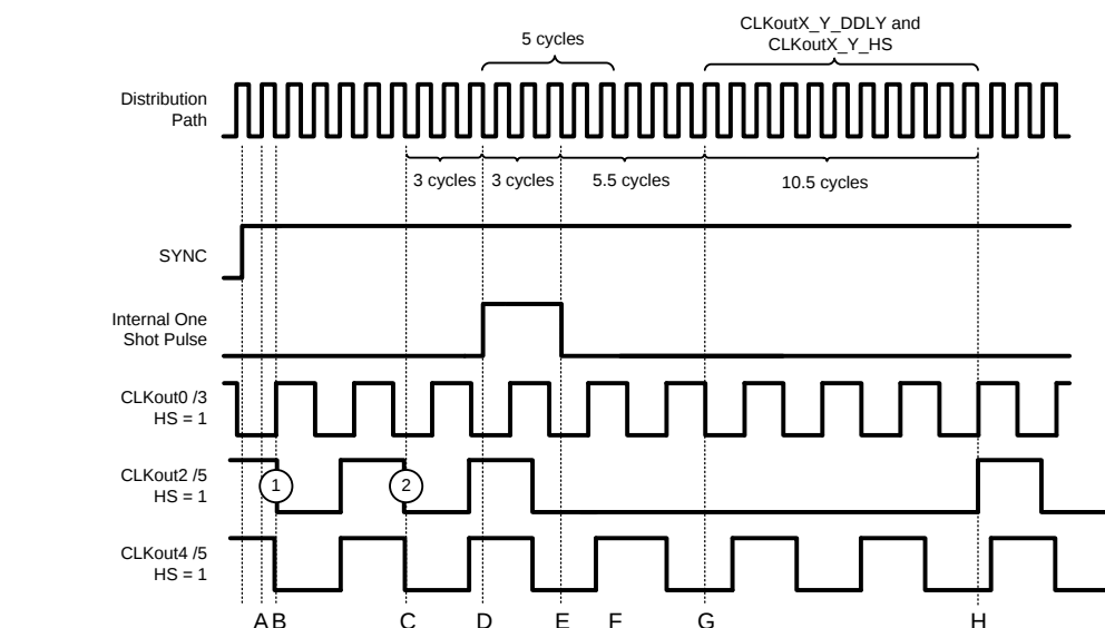
Figure 16. Relative Dynamic Digital Delay Programming Example, 2nd Adjust
