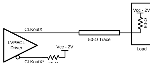
Figure 34. Single-Ended LVPECL Operation, DC Coupling
