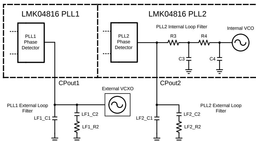
Figure 22. PLL1 and PLL2 Loop Filters
