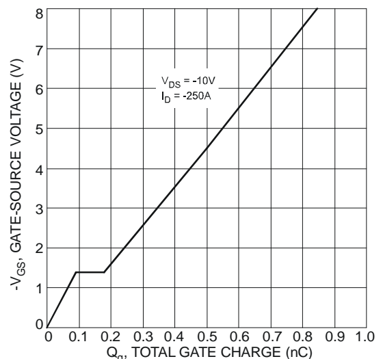
Fig. 12 Gate-Charge Characteristics
