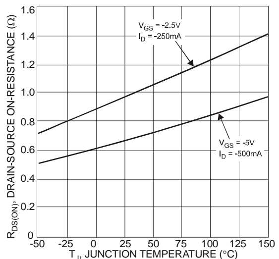
Fig. 6 On-Resistance vs. Temperature
