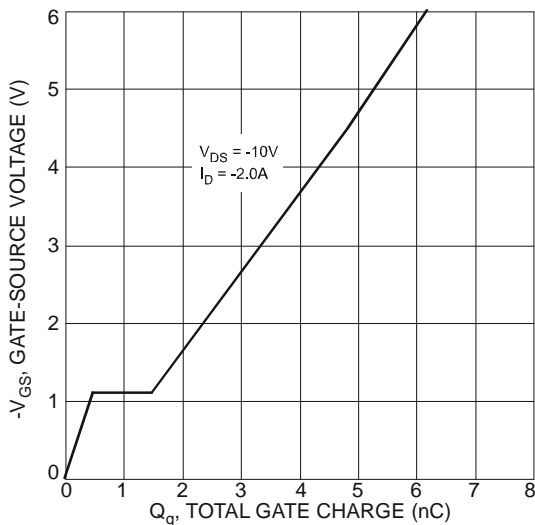
Fig. 11 Gate-Charge Characteristics
