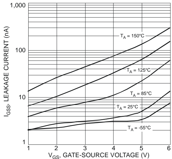
Fig. 10 Gate-Source Leakage Current vs. Voltage
