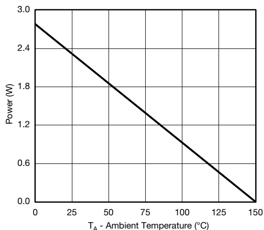
Power, Junction-to-Ambient
